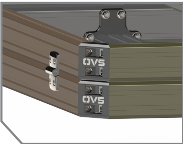
HEAVY-DUTY ALUMINUM CORNER JOINTS
